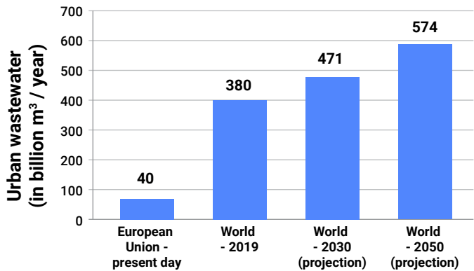
Figure 1: Annual urban wastewater production in Europe and in the world, including projections towards 2050. 29
