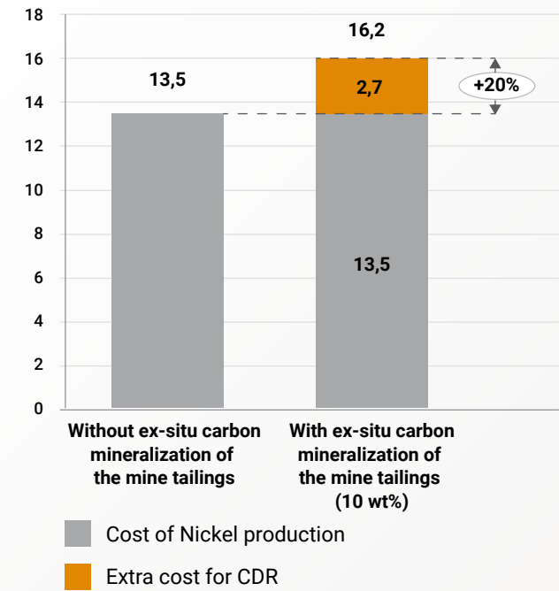
Figure 15 & 16: Costs of Nickel and Platinum Group Metal production with, and without implementing carbon mineralization technology at a rate of 10 wt% in the mined tailings waste products 161
