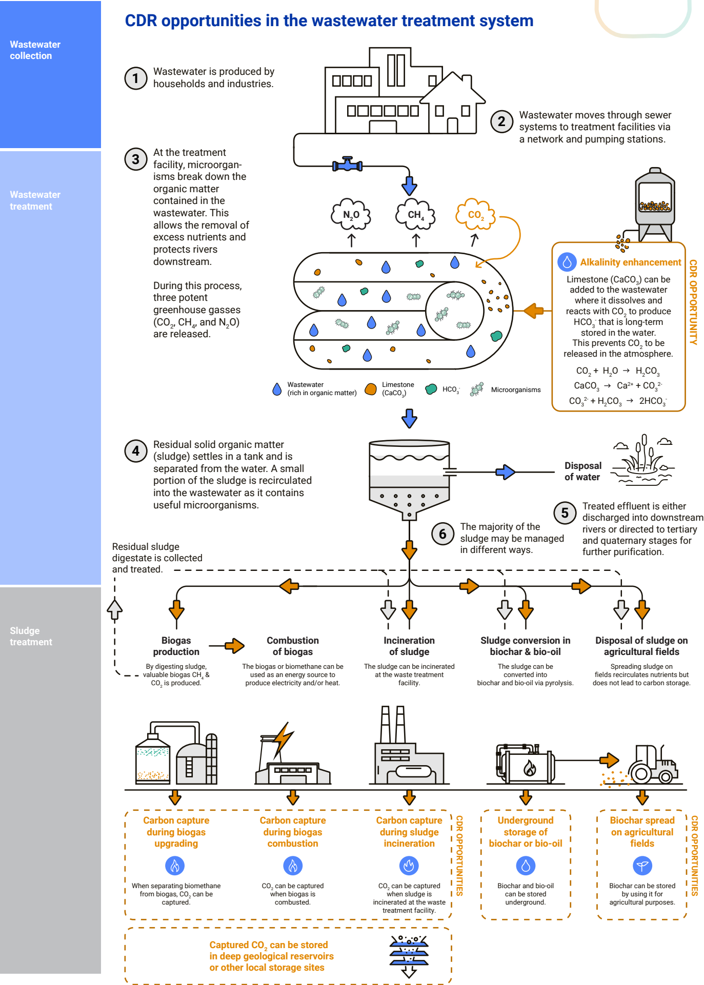
Figure 3: CDR opportunities in the wastewater treatment system.
