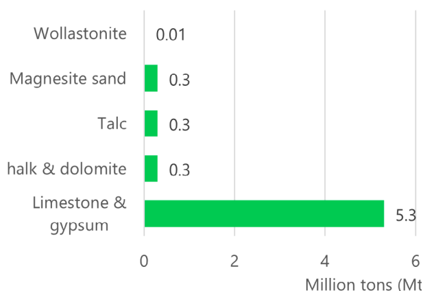
Figure 17. Mineral extraction in Finland in 2023. 64 *No data available for basalt as it is produced only in limited quantities.
