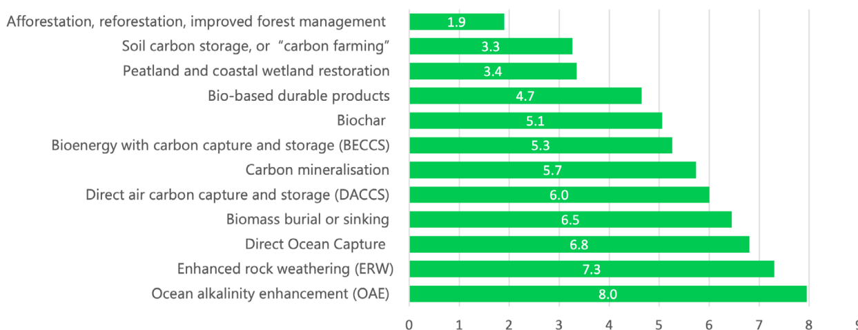
Figure 32. Preferred combination of CDR methods based on the responses of the citizen panel participants in the pre-survey.
