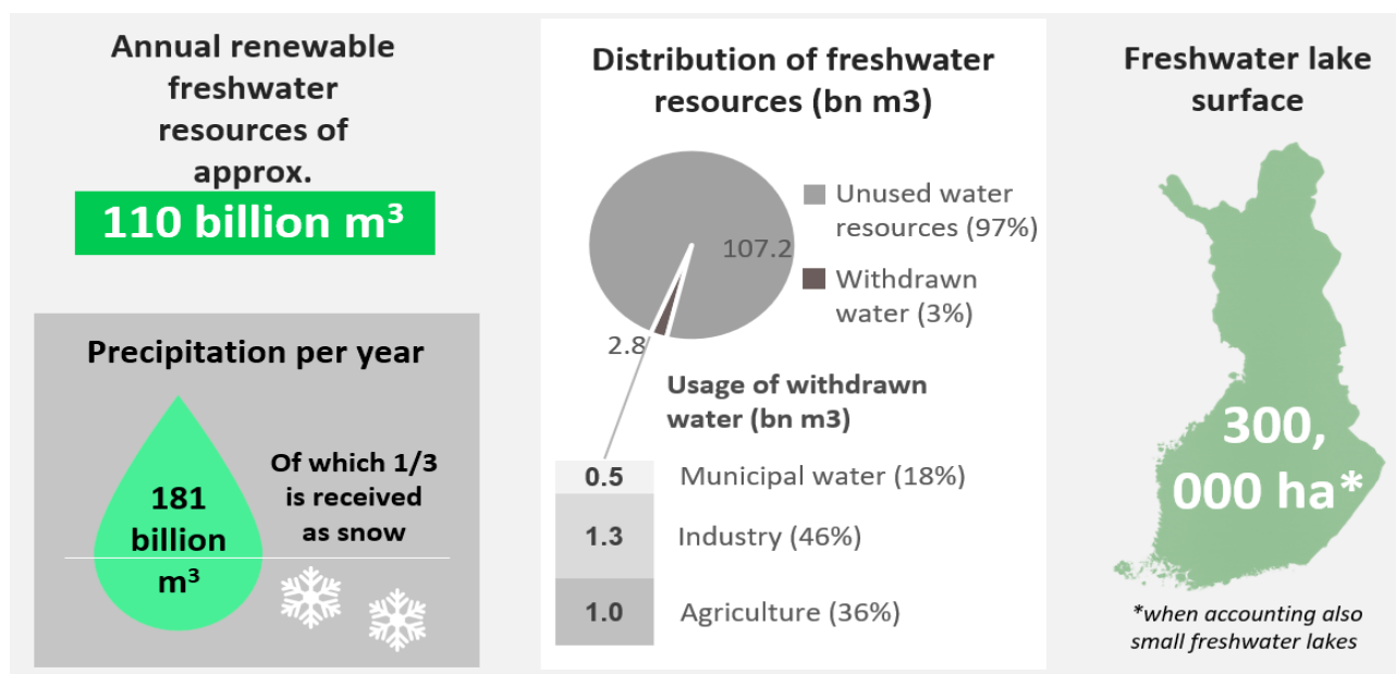
Figure 12. Overview of freshwater resources in Finland.
