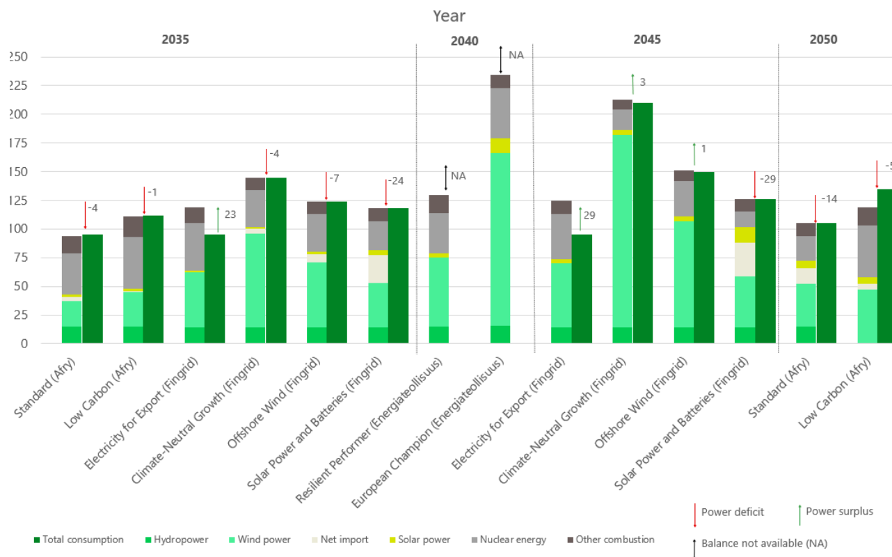
Figure 8. Summary of electricity production scenarios (including imports) by Afry 23 , Energiategollisuus 24 , and Fingrid. 4
