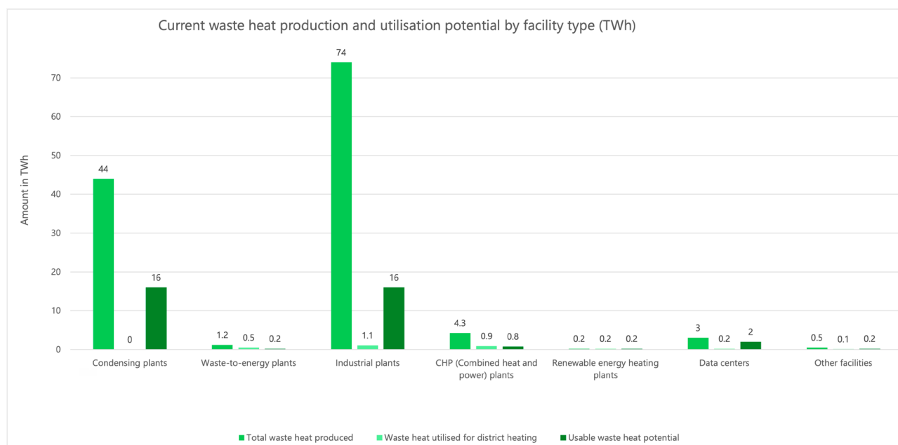
Figure 11. Current waste heat production and utilisation potential by facility type in TWh. 10
