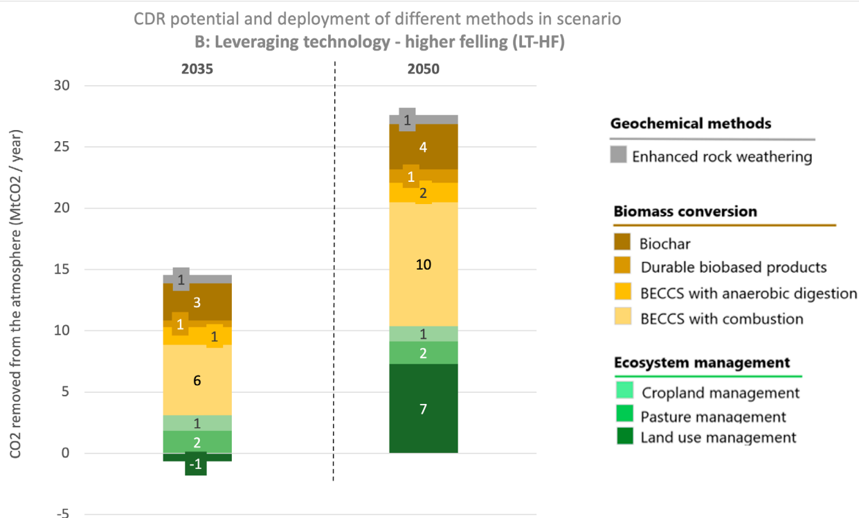
Figure 35. CDR potential of different methods in scenario B. Land use management loses significance as technical CDR methods are included in the calculation. Negative values in this graph represent GHG emissions, indicating that the natural sink operates as a source under scenario B in 2035.
