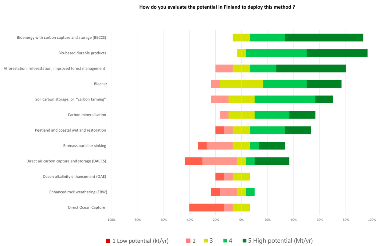
Figure C.1: Answers of the stakeholders in the pre-survey question: How do you evaluate the potential in Finland to deploy this method? In the graph the CDR methods have been ranked according to weighed average, showing the most favoured on the top.
