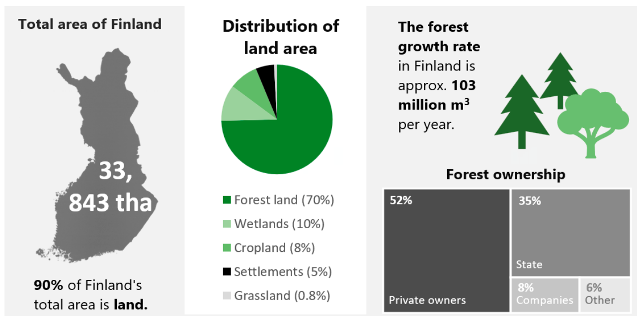
Figure 13. Overview of Finland's land area and forests according to the National Greenhouse Gas Inventory. 21 Species composition of forest land is dominated by pine (less than 66%), followed by spruce (25%) and deciduous trees (10%).
