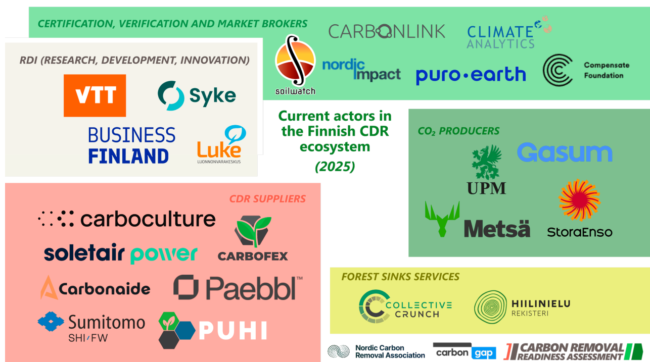
Figure 23. Current main actors in the Finnish CDR ecosystem.
