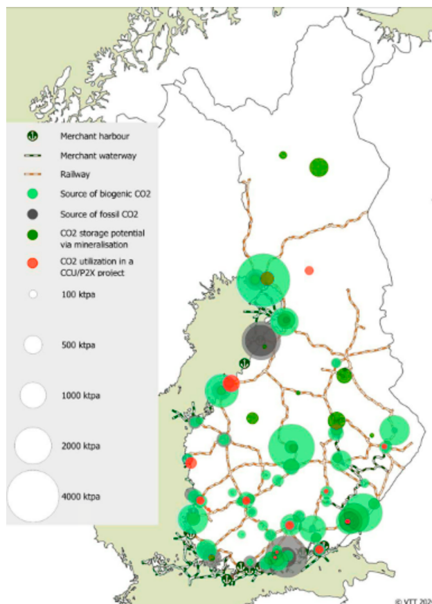
Figure 18. Point sources of CO 2 emissions exceeding 100 ktCO 2 per year. 95
