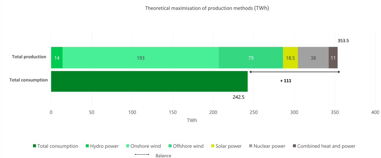
Figure 21. Theoretical maximum capacity of different electricity production methods in 2050.
