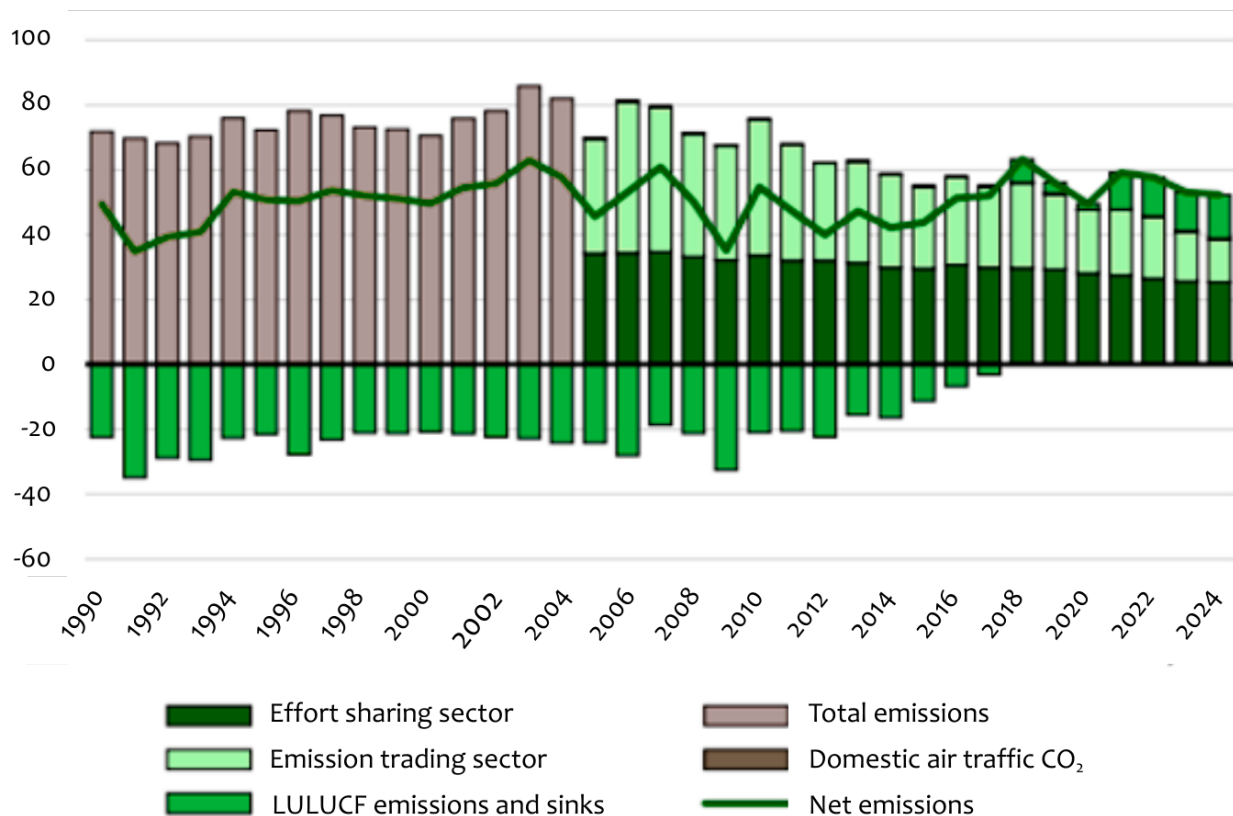
Figure 22. Development of total emissions 1990–2024*. Negative values describe situations where the land use sector was a net sink. Total emissions refer to the combined emissions of the emissions trading and effort sharing sectors. From 2005 onwards, total emissions, excluding the LULUCF sector, have been divided into the effort-sharing and emissions-trading sectors. Source: Ministry of the Environment. 109 *The 2024 data are preliminary estimates.
