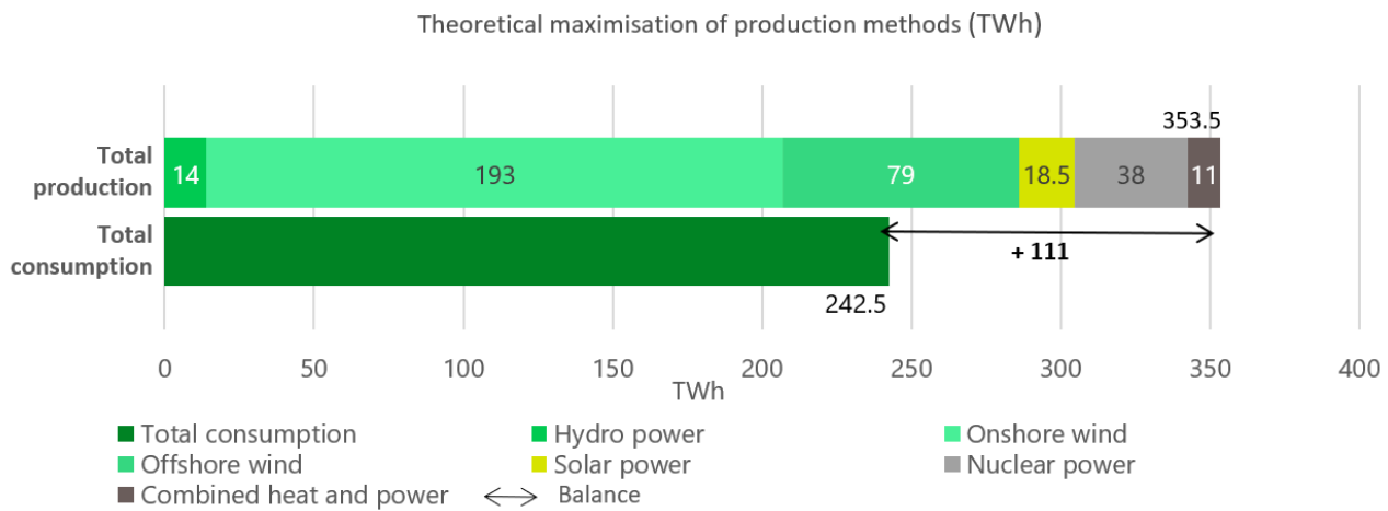
Figure 9. Projection of theoretical maximisation of electricity production methods in 2045 based on the Fingrid climate growth scenario.
